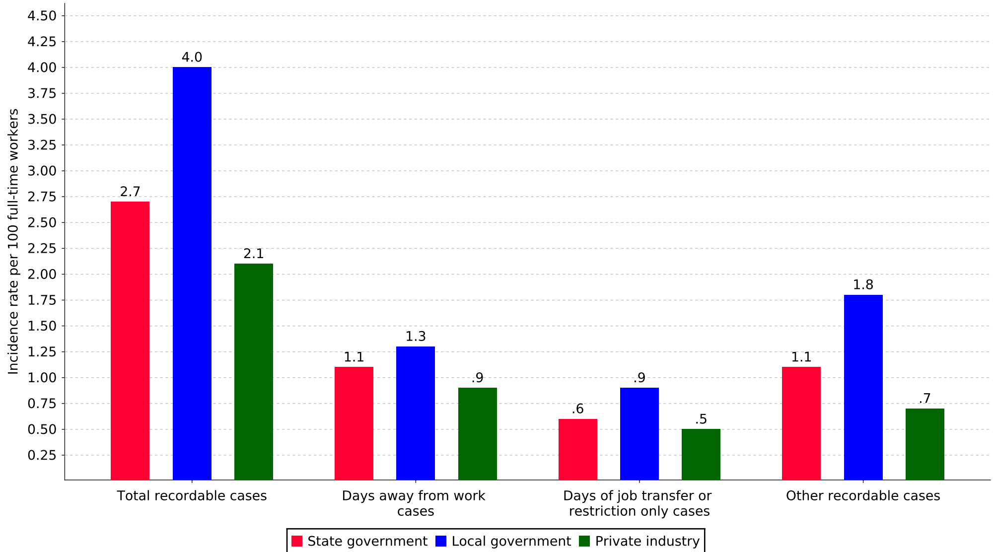
Nonfatal occupational injury and illness incidence rates by case type and ownership, South Carolina, 2020 [SOURCE : U.S. Bureau of Labor Statistics, U.S. Department of Labor, 2021]
